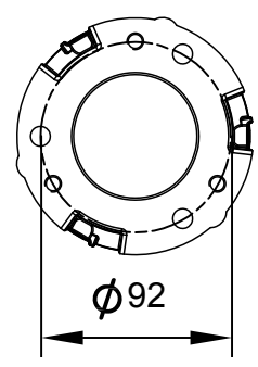
Installation template
